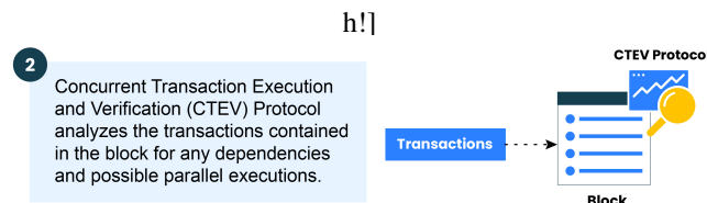
Figure 12: CTEV analyzes the transactions in the block
