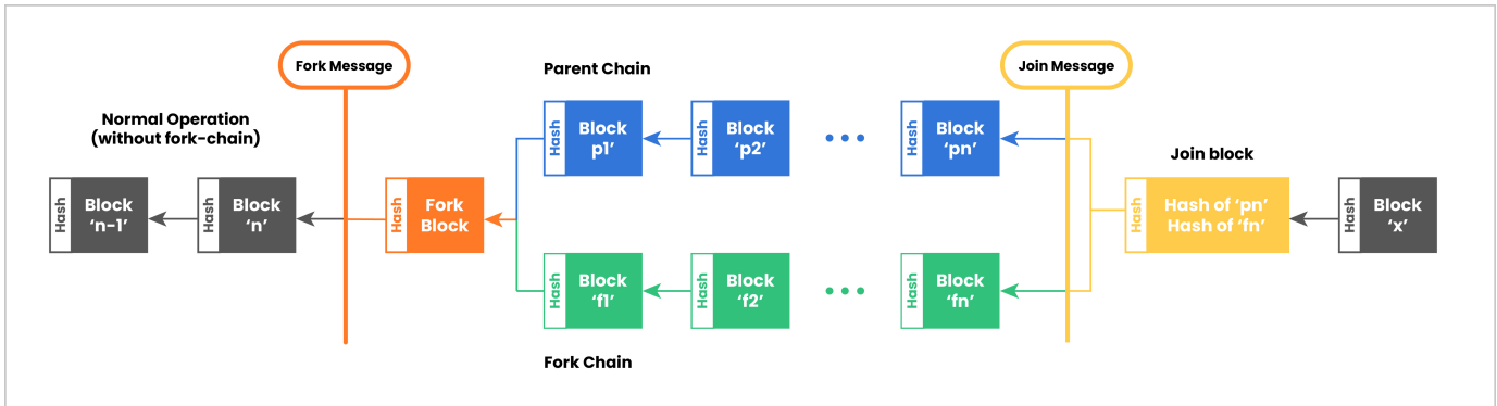
Figure 10: Fork fchain synchronization
